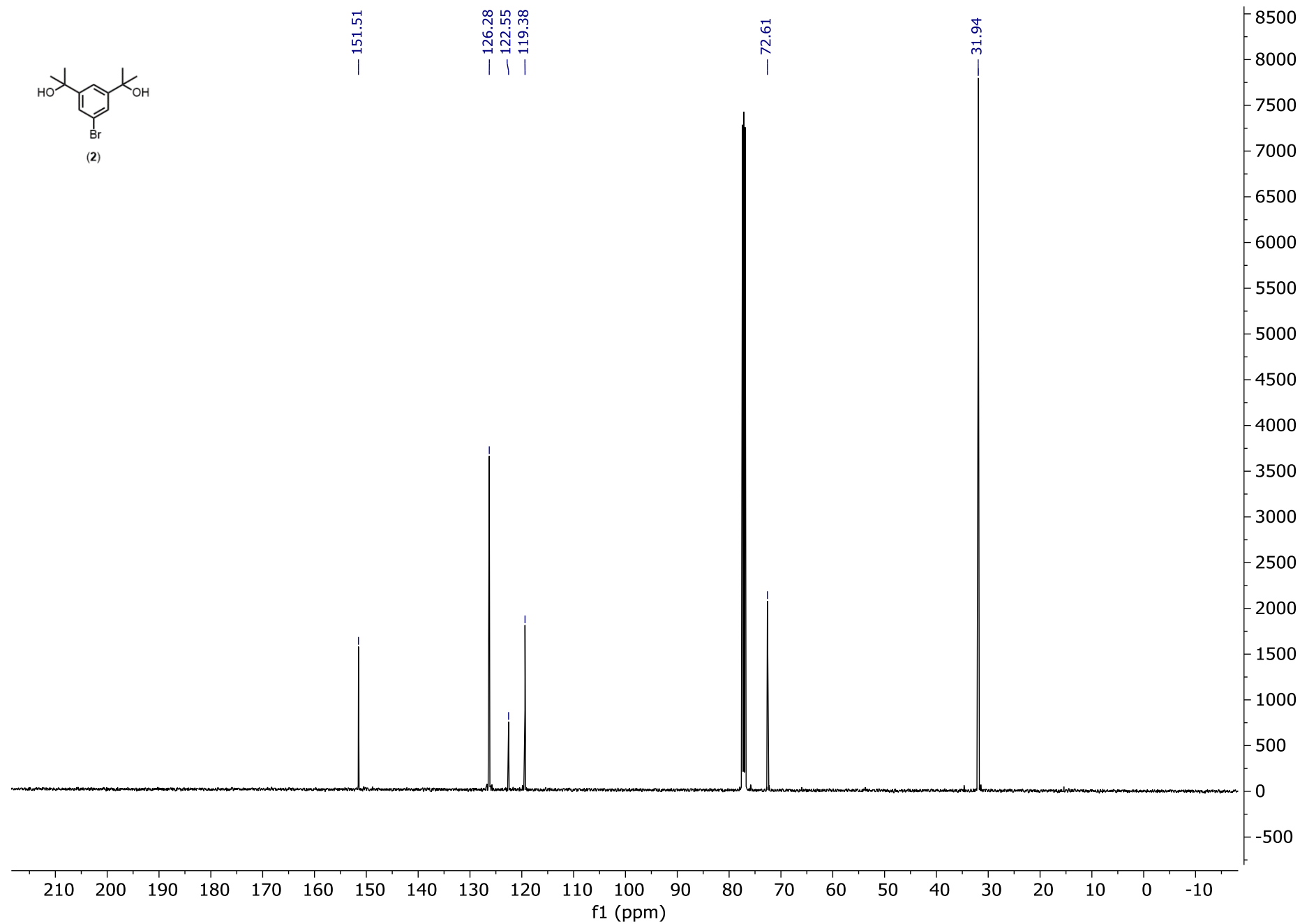
^{13}\text{C} NMR of 1-bromo-3,5-bis(1-hydroxy-1-methylethyl)benzene ( 2 ) (126 MHz, \text{CDCl}_3 )
